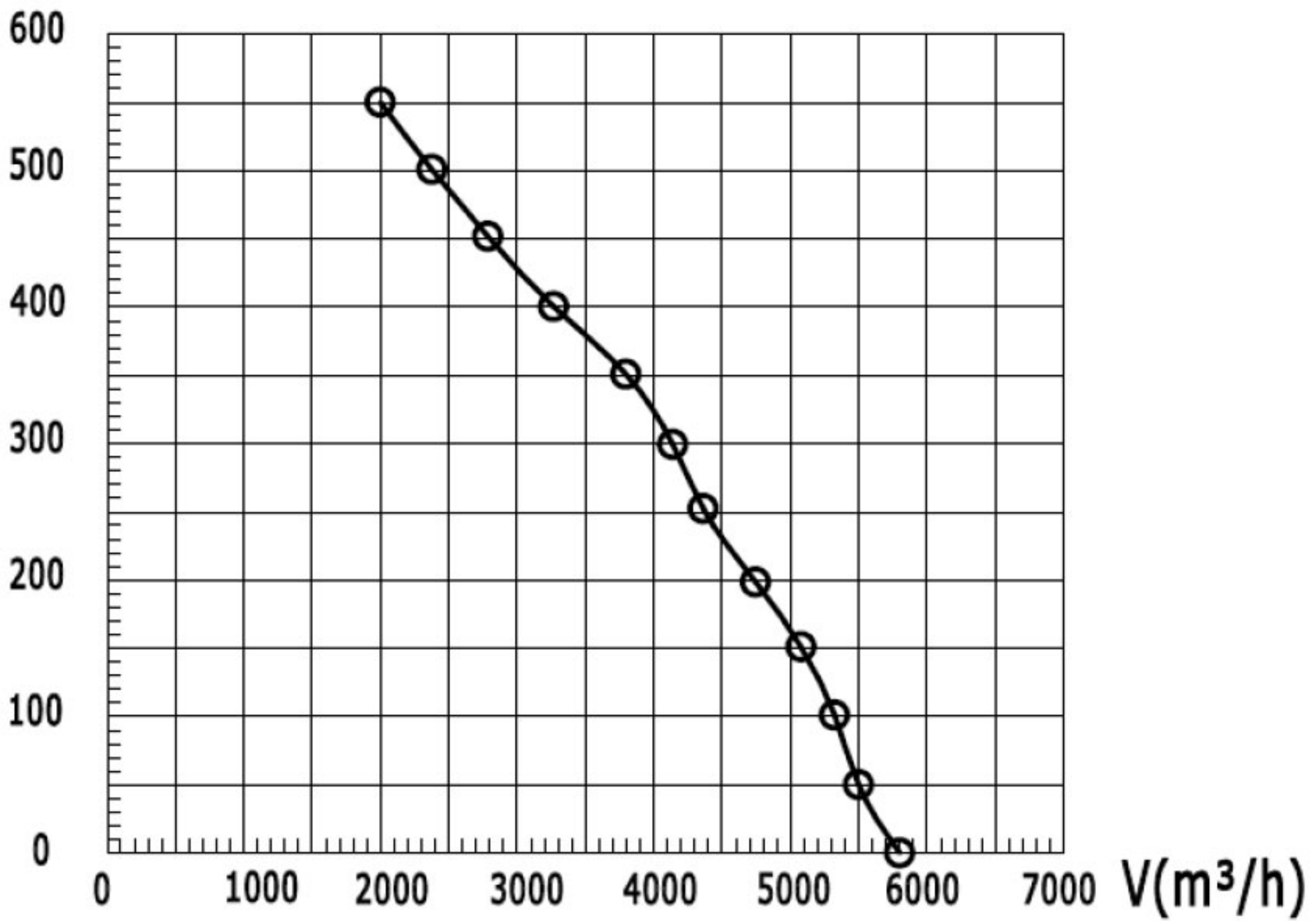
Airflow curves
